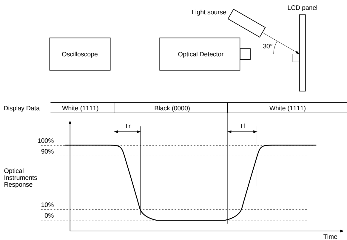
Fig. 3. Measurement system-3
